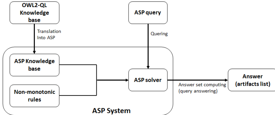
Figure 4: Query answering process for OWL knowledge base and ASP solver.
