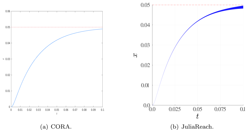
Figure 14: Brake (BRKDC01): Reachable sets for x over time.
