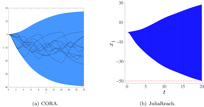
Figure 9: PLAA01: Reachable sets of x_1 plotted over time. CORA additionally shows possible trajectories.
