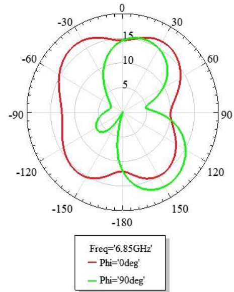
Fig. 7. E-plane and H-Plane Radiation Pattern of HMSA at 6.85 GHz
