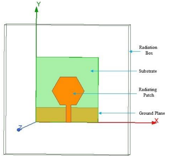
Fig. 2. Geometry of proposed antenna structure
