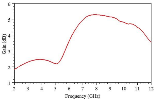
Fig. 6. Gain variation verses Frequency of HMSA
