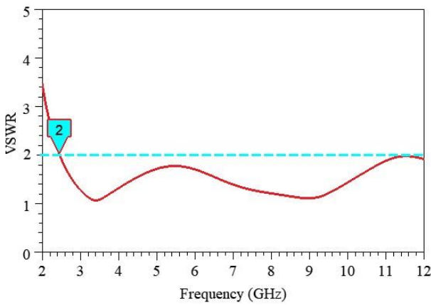
Fig. 5. VSWR verses Frequency of HMSA
