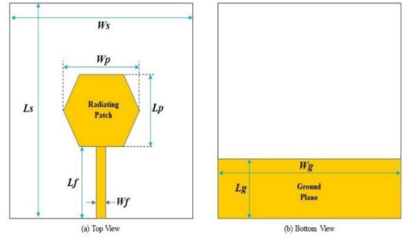
Fig. 3. Design details of dimensions of HMSA
