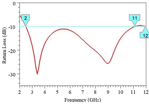
Fig. 4. Return loss verses Frequency of HMSA
