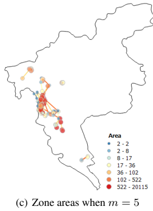
Figure 8. Zone areas of UHIs in different magnitudes associate with their trajectories between July 31 and August 6.
