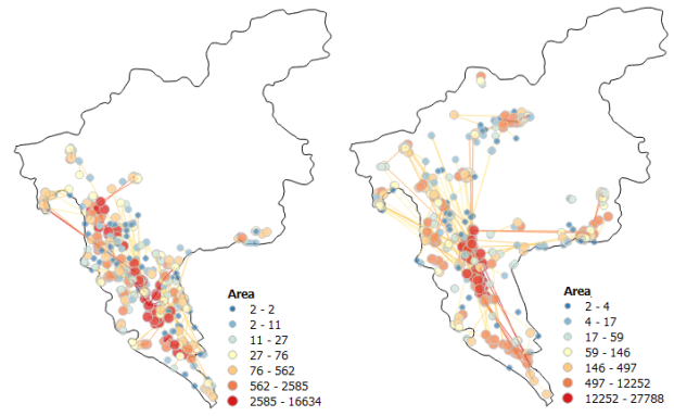
(c) Zone area in 09/25-10/01
