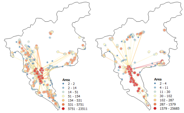
(e) Zone area in 11/20-11/26
