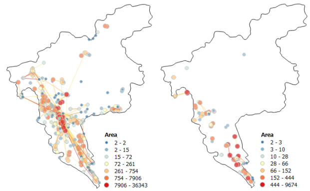
(a) Zone area in 07/31-08/06
