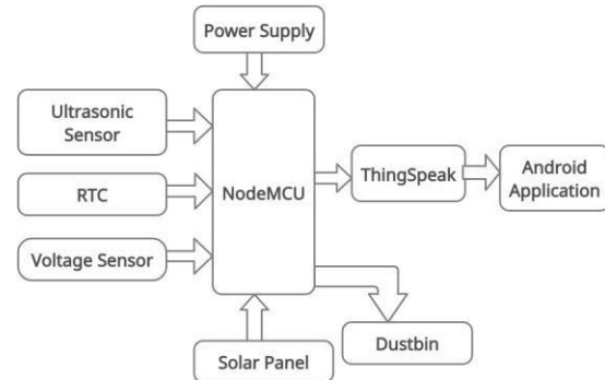
Fig 4.1 Architecture of smart dustbin
