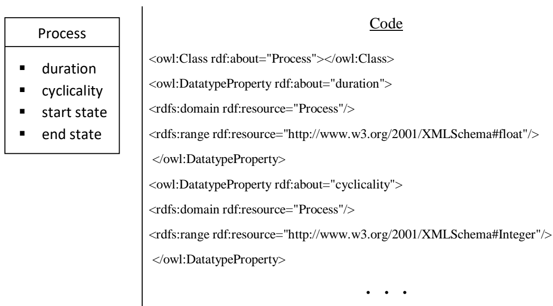
Fig.2. The “Process” class.
