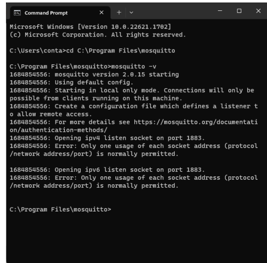
Fig. 8. Mosquitto - version 2.0.15 starting
