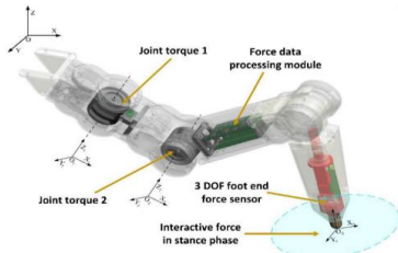
Figure.3. Joints using U- Brackets [2]
