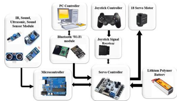
Fig.10. Electrical throng of total project.
