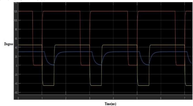
Figure.5. Leg 1, 3 and 5 Angle vs. time wave shapes in MATLAB.
