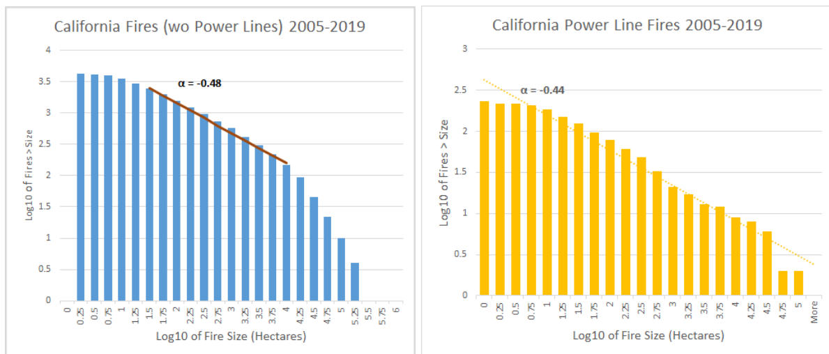
Fig. 2 CAL FIRE perimeter data for wildfires attributed to power line ignitions. 2007 and 2017 fire attributions are corrected with CAL FIRE and CPUC assessments. The trendlines are a guide to the eye, rather than a best fit and shows how power law exponents would appear. Deviations from power law behavior appear above 30,000 acres (without power lines) and 80,000 acres for power line fires.
