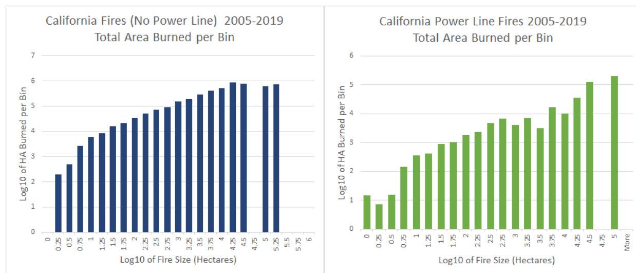
Fig 3 Total area burned per logarithmic bin for California wildfires 2005 to 2019, calculated by multiplying logarithmic mean of bin by number of wildfires in the bin. Power line related wildfires are compared against full sample with non-power line wildfires removed.
