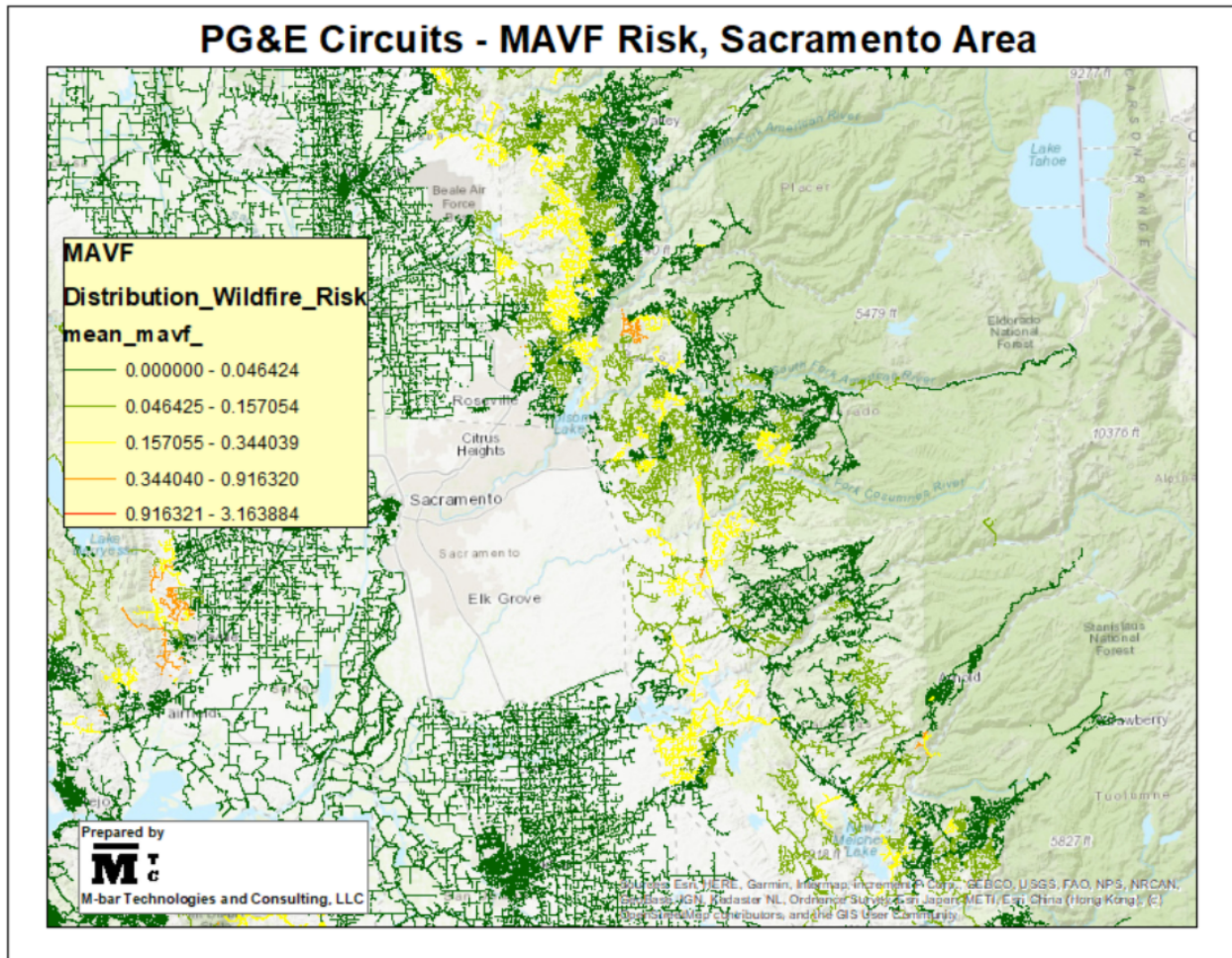
Fig 4 PG&E Wildfire Distribution Risk Model (WDRM) v2 risk estimates for circuits in the Sacramento/Lake Tahoe area. Green areas. Note that the areas of greatest risk tend to be greater nearer population centers, and drop to lower values for more remote areas.
