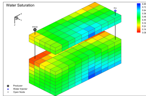
Figure 21: Water saturation in the reservoir after 500 days
