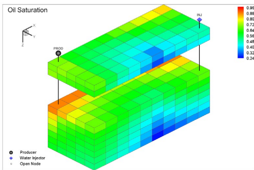
Figure 19: Oil saturation in the reservoir after 500 days.
