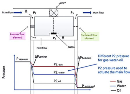
Figure 5: A simplified sketch of the flow paths in AICV and pressure changes inside for different fluids (Anuththara et al. 2023).
