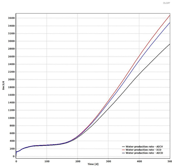
Figure 14: Water production rate for 500 days for ICD, AICD, and AICV.
