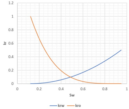
Figure 9: Relative permeability curves.
