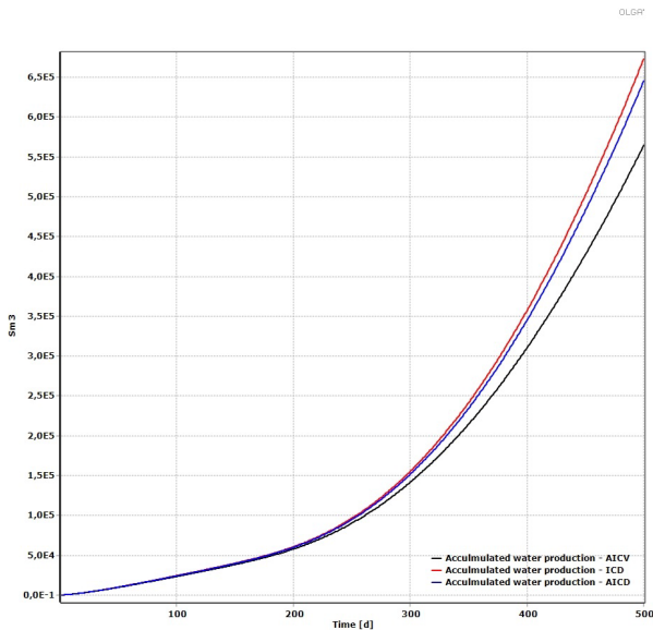
Figure 15: Accumulated water production for ICD, AICD, and AICV for 500 days.
