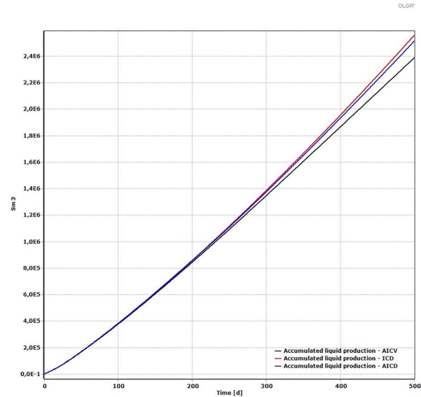
Figure 17: Total accumulated liquid production for 500 days for ICD, AICV, and AICD.
