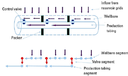
Figure 2: Schematic of a multisegmented well model (Moradi et al. , 2022a).
