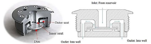
Figure 4: Schematic diagram of Statoil's RCP valve (Anuththara et al. , 2023).
