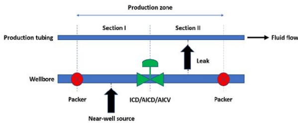
Figure 11: Layout for one production zone.
