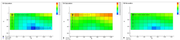
Figure 20: Oil saturation in the horizontal layer around the top, middle, and bottom laterals after 500 days.
