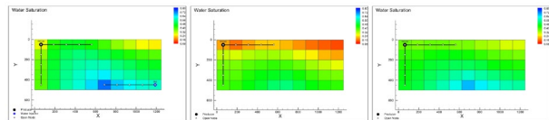
Figure 22: Water saturation in the horizontal layer around the top, middle, and bottom laterals after 500 days.
