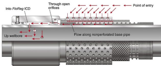
Figure 3: Orifice-type ICD and its flow path (Mathiesen et al. , 2014).
