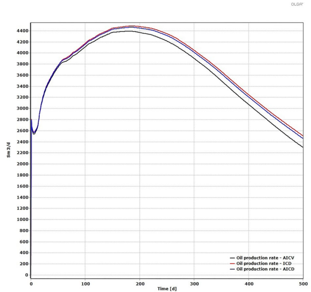
Figure 12: Oil production rate for ICD, AICD, and AICV models.
