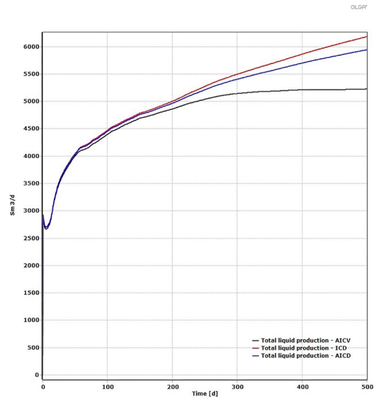
Figure 16: Total liquid production rates for 500 days for ICD, AICD, and AICV.
