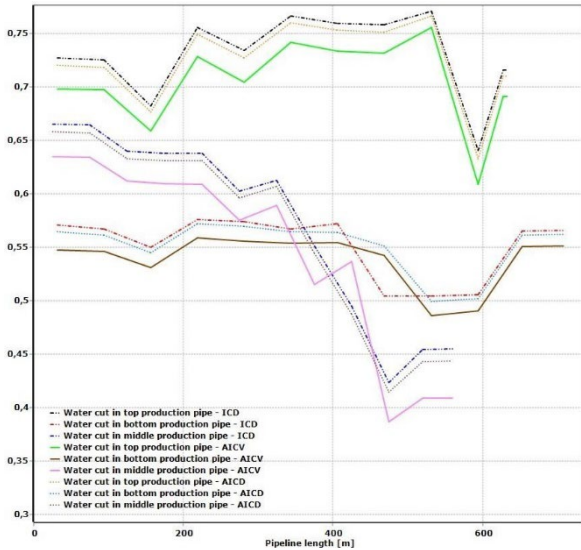
Figure 18: Water cut (WC) variation along all the laterals for ICD, AICD, and AICV.
