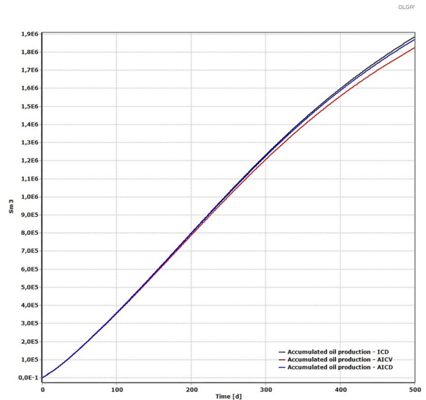
Figure 13: Accumulated oil production over 500 days for ICD, AICD, and AICV.
