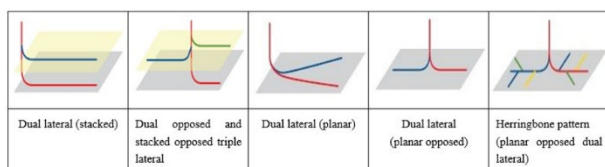
Figure 1: Types of different multilateral wells (Flatern, 2021).
