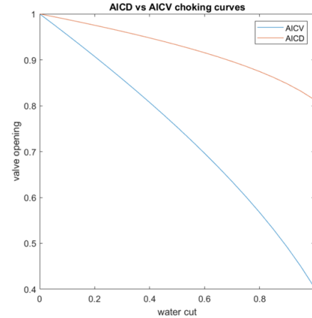
Figure 6: Choking functionality comparison between AICV and AICD.
