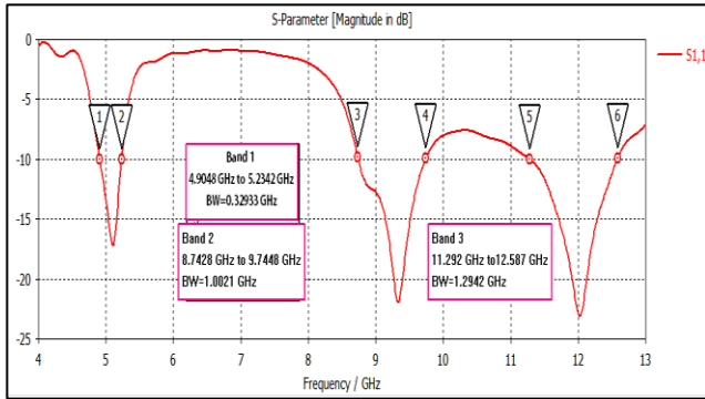
Figure 4: Bandwidth
