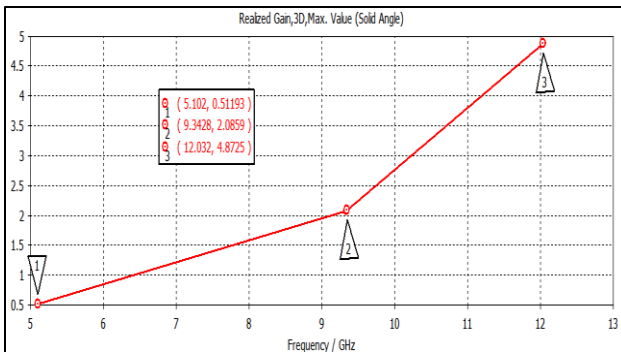
Figure 6: Realized gain
