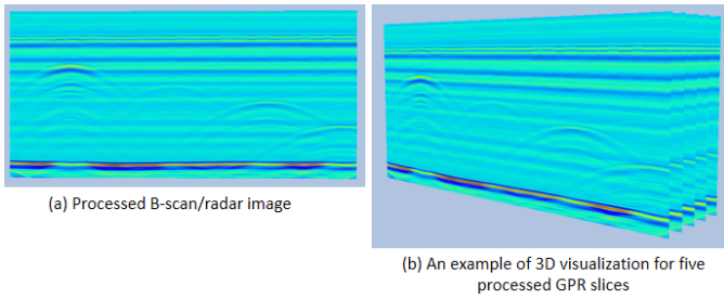
Fig. 6. 3D representation using as reference images radar.
