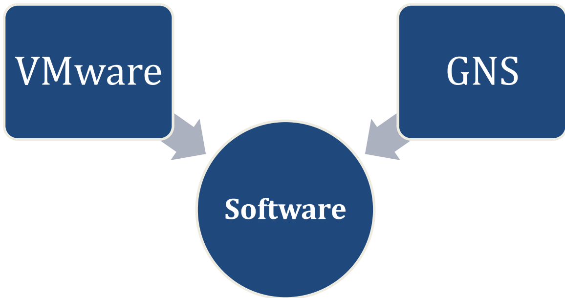
Fig.3 Software Analysis
